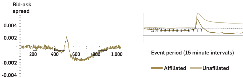
■ Figure 5. Simulations of the reaction of a bid-ask spread to a market event occurring at T=512 using the model of Equations (6), (11-12) with time-changing rates of arrival of traders provided by Equation (16)
