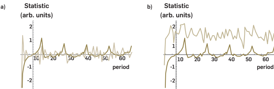
a) The sample with best-fitted values of parameter vector \theta , r^2 \approx 30\% . b) Sample weighted according to posterior distribution, r^2 \approx 70\% . The graph for model dynamics is shifted upwards for clarity of presentation
